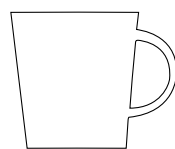
Lomond Fine Bone China 0.32L Height 94mm Top Diameter 88mm
