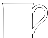
Bute Fine Bone China 0.3L Height 85mm Top Diameter 82mm
