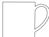
Orkney Fine Bone China 0.35L Height 91mm Top Diameter 88mm
